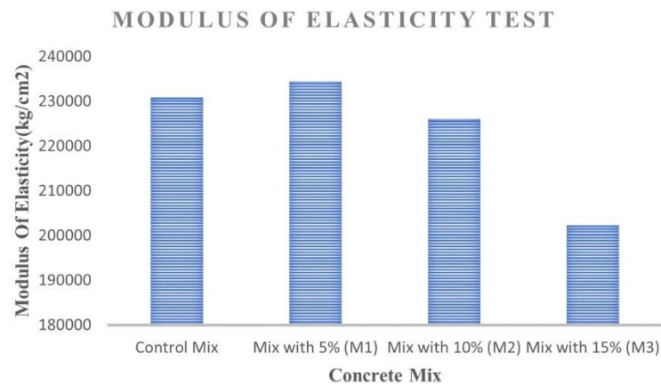
Fig.12 - Variation of the Modulus of Elasticity for an age of 28 days.
