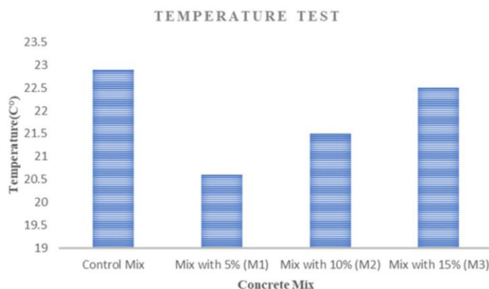
Fig. 10 - Temperature variation for each concrete mix
