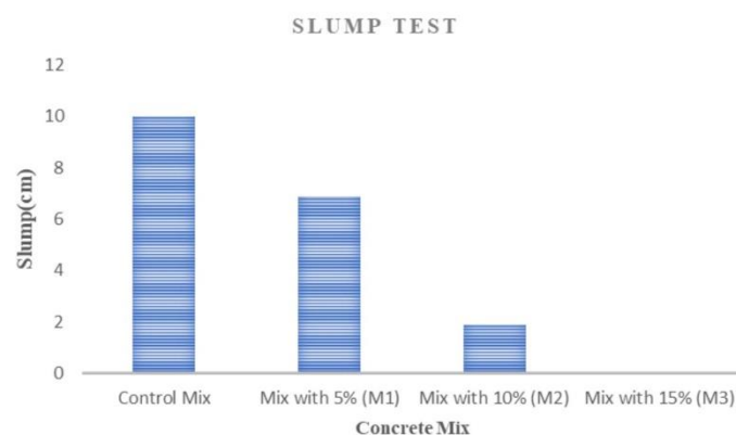
Fig. 7 - Slump Variation according to the proportion
