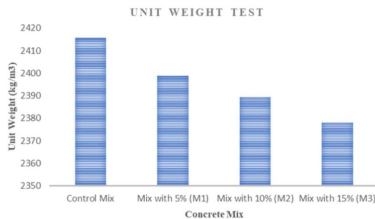
Fig. 9 - Variation of Unit Weight for each percentage of addition
