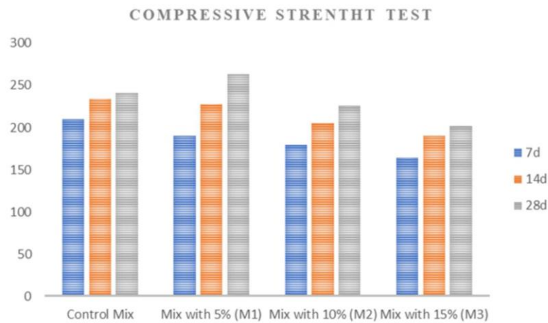
Fig. 11- Concrete resistance for each percentage of addition at 7d,14d,28d.
